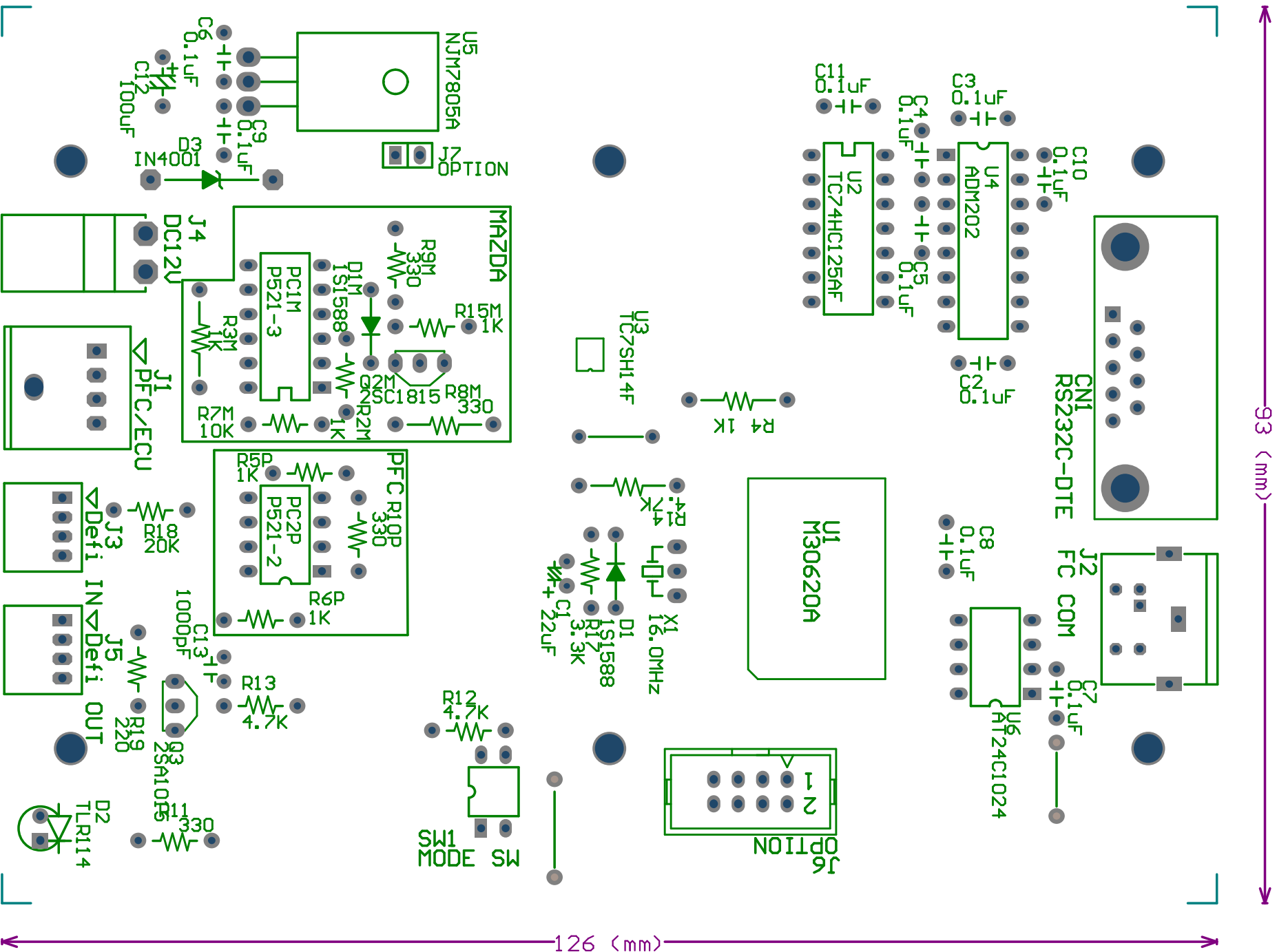
PCB Sanhayato 43K, Chassis TAKACHI SU-140
