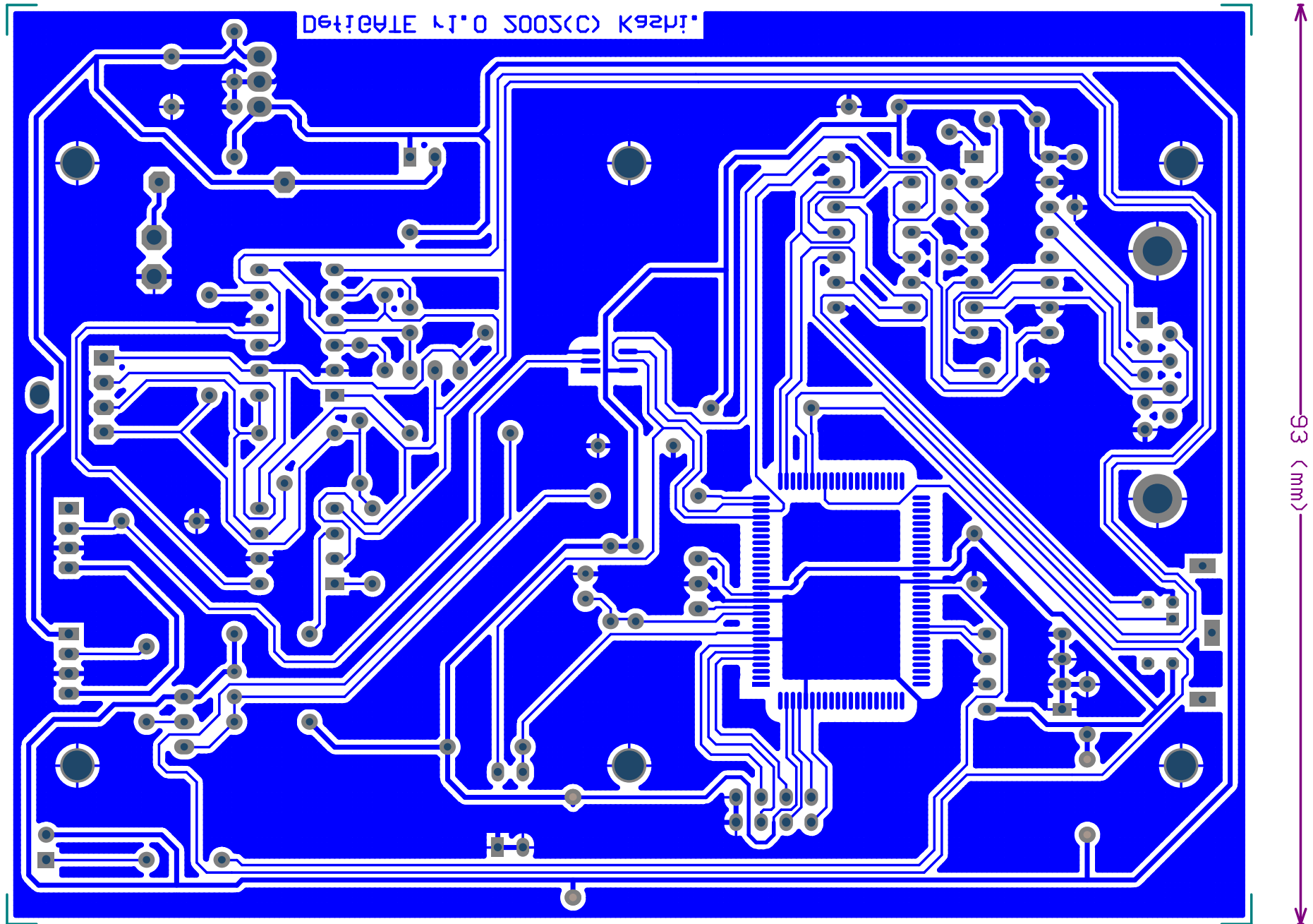
PCB Sanhayato 43K, Chassis TAKACHI SU-140
